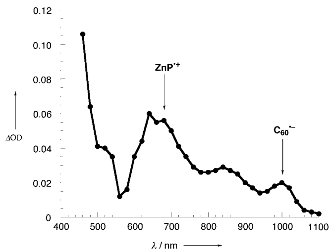
Figure 1. Nanosecond time-resolved transient absorption spectrum of ZnP-NHCO-C 60 excited at 532 nm in THF (absorption ratio of ZnP : C 60 = 3:1).
